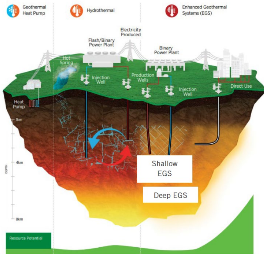
Figure 2: Diversity of geothermal resources and applications
